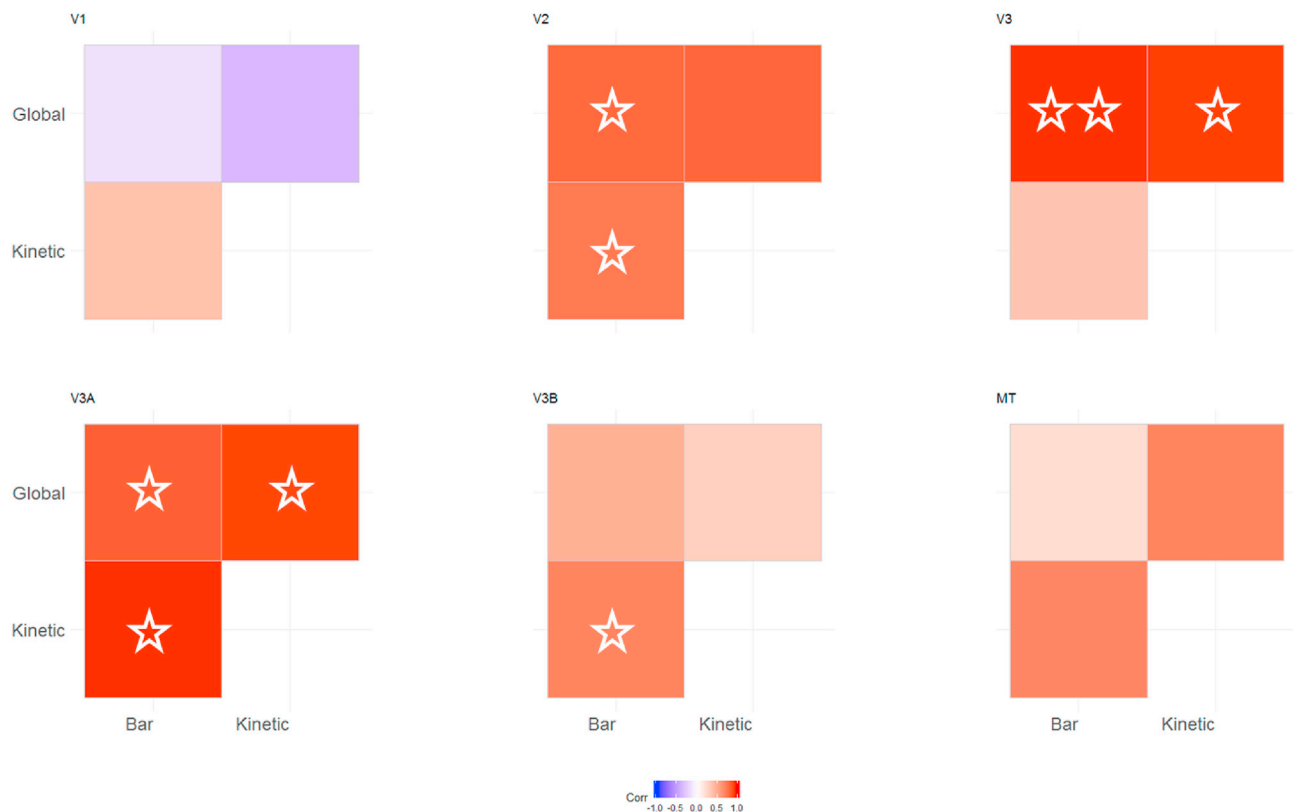
Fig. 3. Correlation matrices comparing pRF polar angles between stimulus conditions in Experiment 1. The colour of each cell indicates the strength and sign of each vertex-wide correlation in polar angle. Circular correlations were calculated for each participant, then Z transformed and averaged across participants (as in (Haas and Schwarzkopf, 2018)). The symbols indicate whether the average correlation in individual cells is significantly different from zero (uncorrected). One star = p < 0.05 . Two stars = p < 0.001 .
