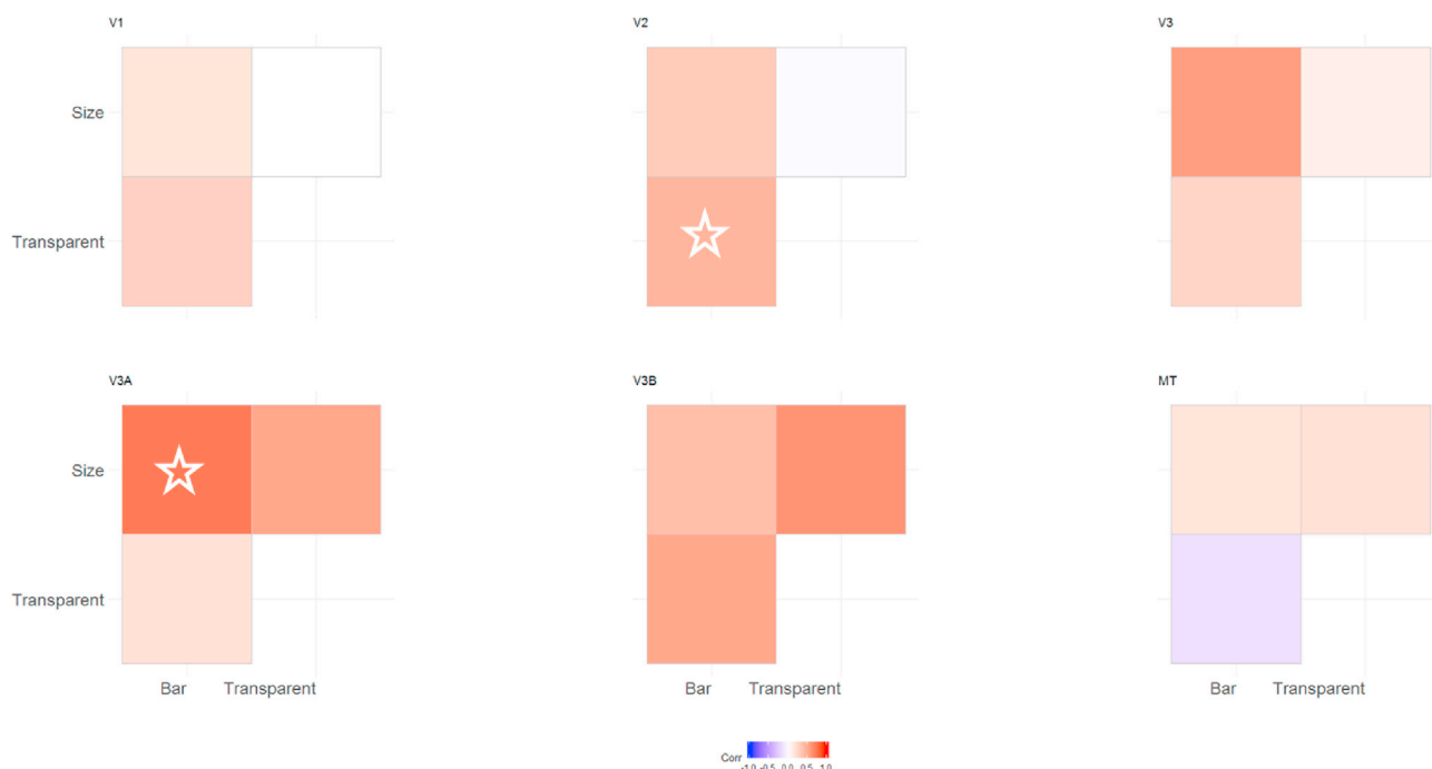
Fig. 8. Correlation matrices comparing pRF polar angles between stimulus conditions in Experiment 2. The colour of each cell indicates the strength and sign of each vertex-wide correlation in polar angle. Circular correlations were calculated for each participant, then Z transformed and averaged across participants (as in (Haas and Schwarzkopf, 2018)). The symbols indicate whether the average correlation in individual cells is significantly different from zero (uncorrected). One star = p < 0.05 . Two stars = p < 0.001 . Note: one participant did not have enough data for valid correlations in the size-defined condition in V3B and MT, and so their data was not used for the average calculation).
